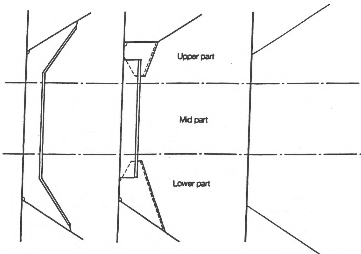
Non - typical transverse frame in cargo hold Thickness gauging area (A)
