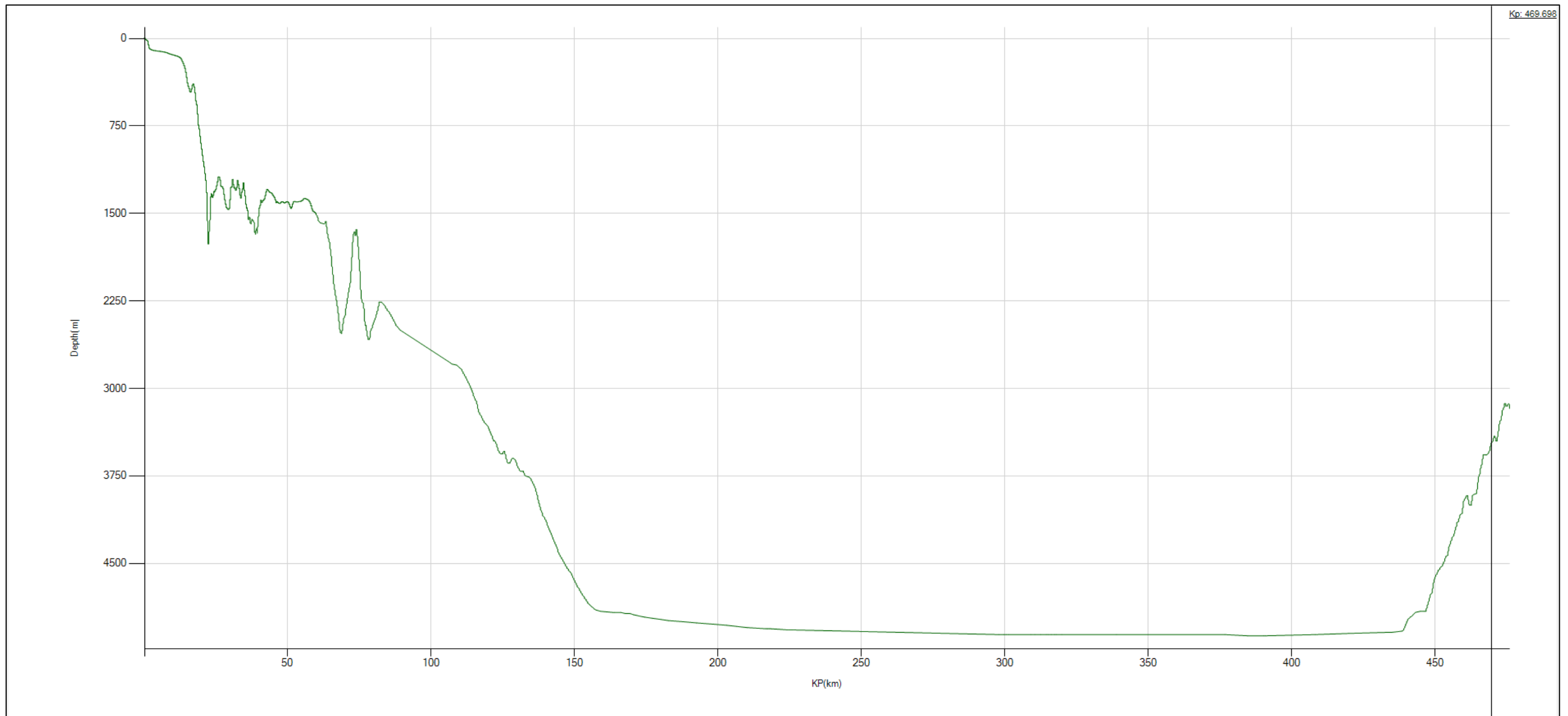
Figure 1 EQUIANO Depth Profile in Portugal waters Segment 1 BMH @ KP 0.000 to PRT EZ @ KP 469.698
